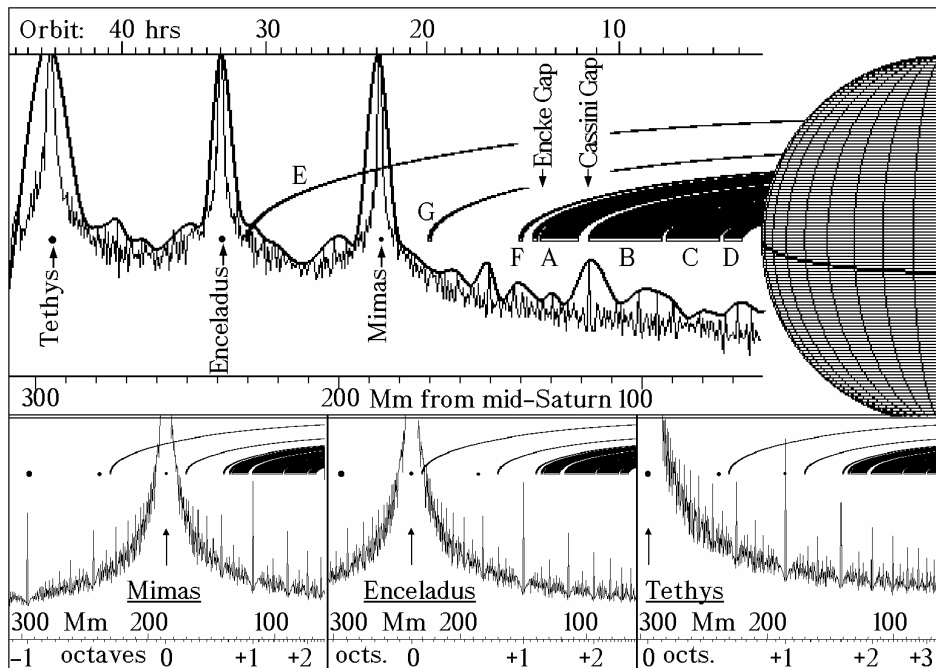
16 - Saturn rings A-G, harmonicities curves from satellites
